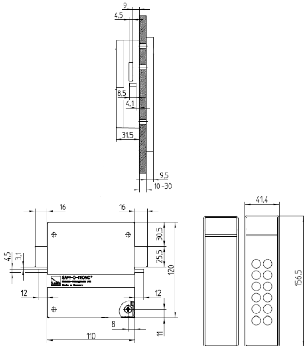
Picture 9.1 – Technical dimensions - Top: Side view with door (gray), outdoor unit (right) and indoor unit (left) - Bottom: Indoor unit (left) and outdoor unit (right)
