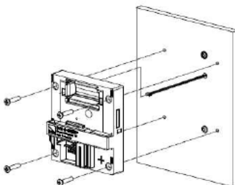
Picture 2.4 – Installation of the indoor unit
