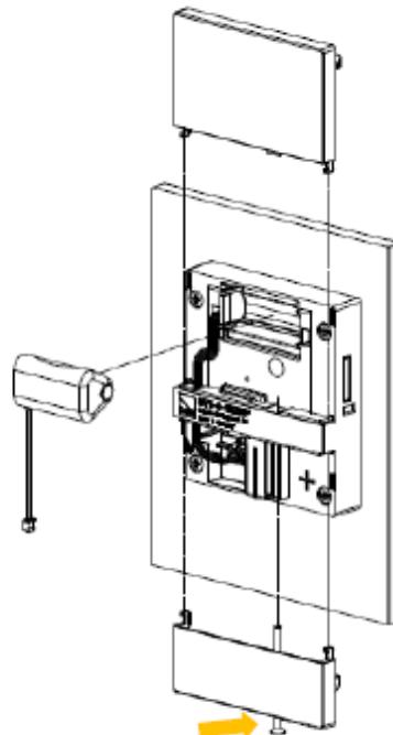
Picture 2.5 – Mounting the indoor unit
