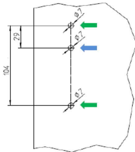
Picture 2.1 – Required holes for the external unit
