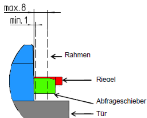
Picture 2.7 – Frame position (dashed line) for correct function of the query slider. Bolt (red), query slider (green), door (gray), and lock (blue)
