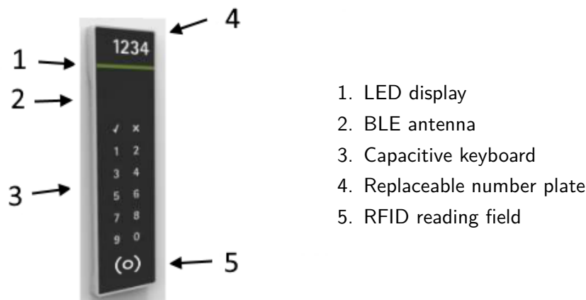
Picture 1.1 – LSW with all functions
